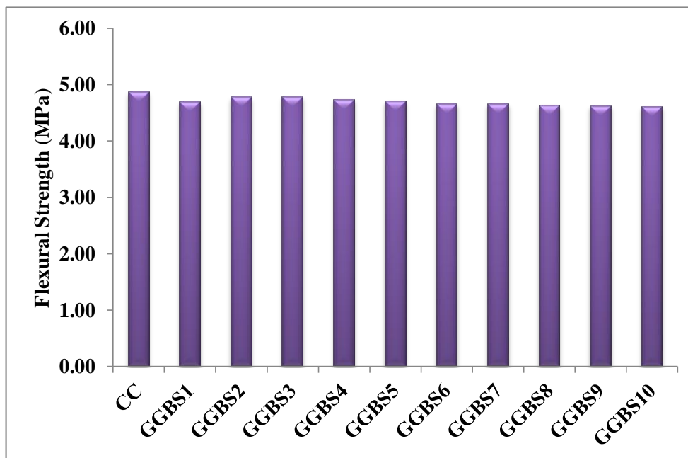
Figure 4. Flexural Strength of GGBS based Concrete
