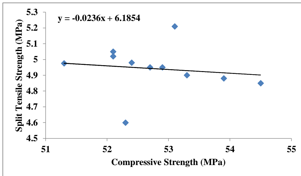
Figure 3. Regression Analysis of Split Tensile Strength vs Compressive Strength
