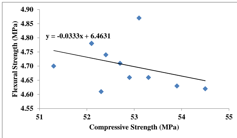
Figure 5. Regression Analysis of Flexural Strength vs Compressive Strength
