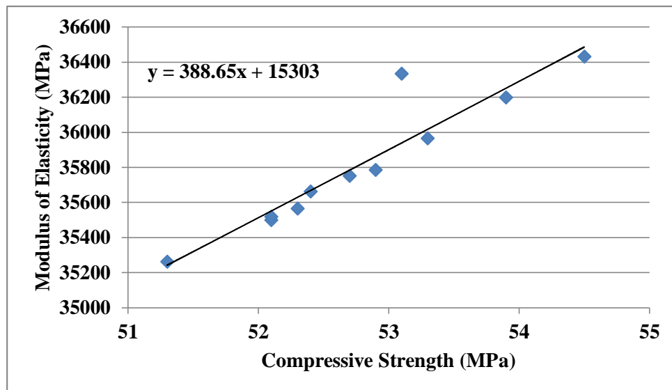
Figure 7. Regression Analysis of Modulus of Elasticity vs Compressive Strength
