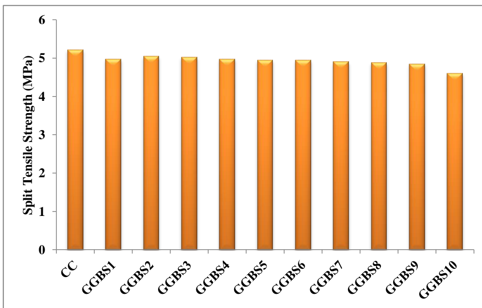
Figure 2. Split Tensile Strength of GGBS based Concrete
