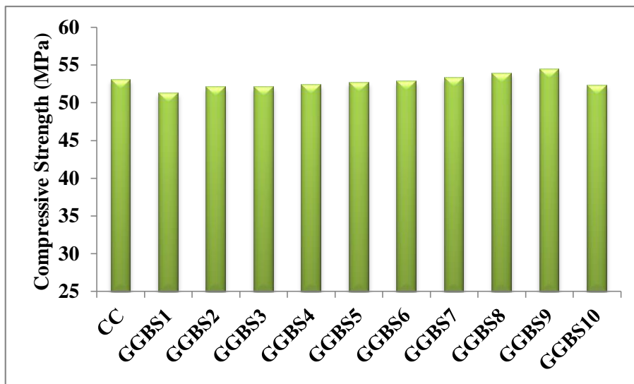
Figure 1. Compressive Strength of GGBS based Concrete
