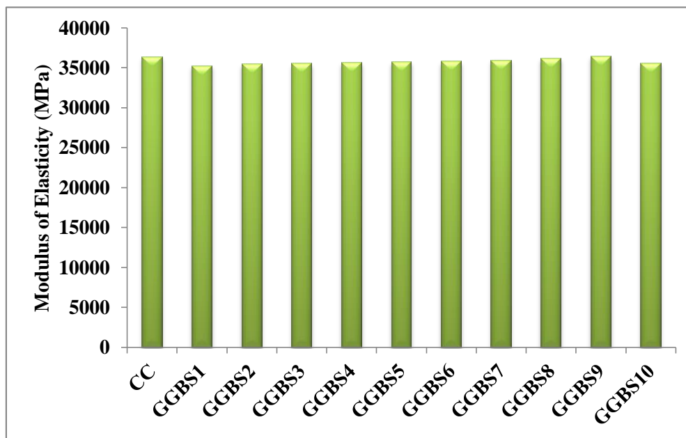
Figure 6. Modulus of Elasticity of GGBS based Concrete
